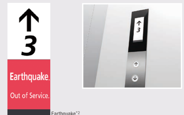
Earthquake* 2
