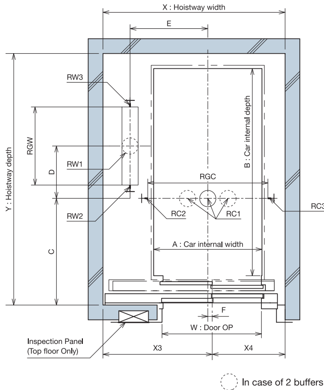
Hoistway dimension and Pit reaction loading
