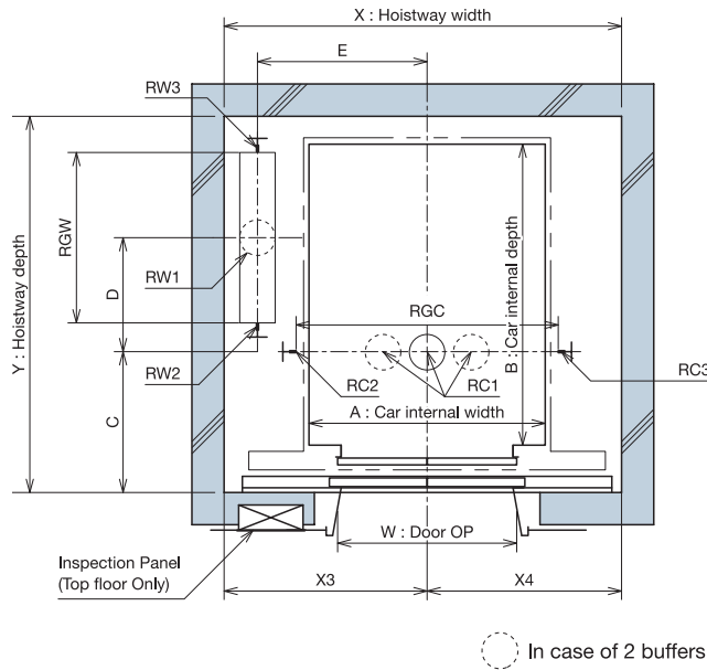
Hoistway dimension and Pit reaction loading
